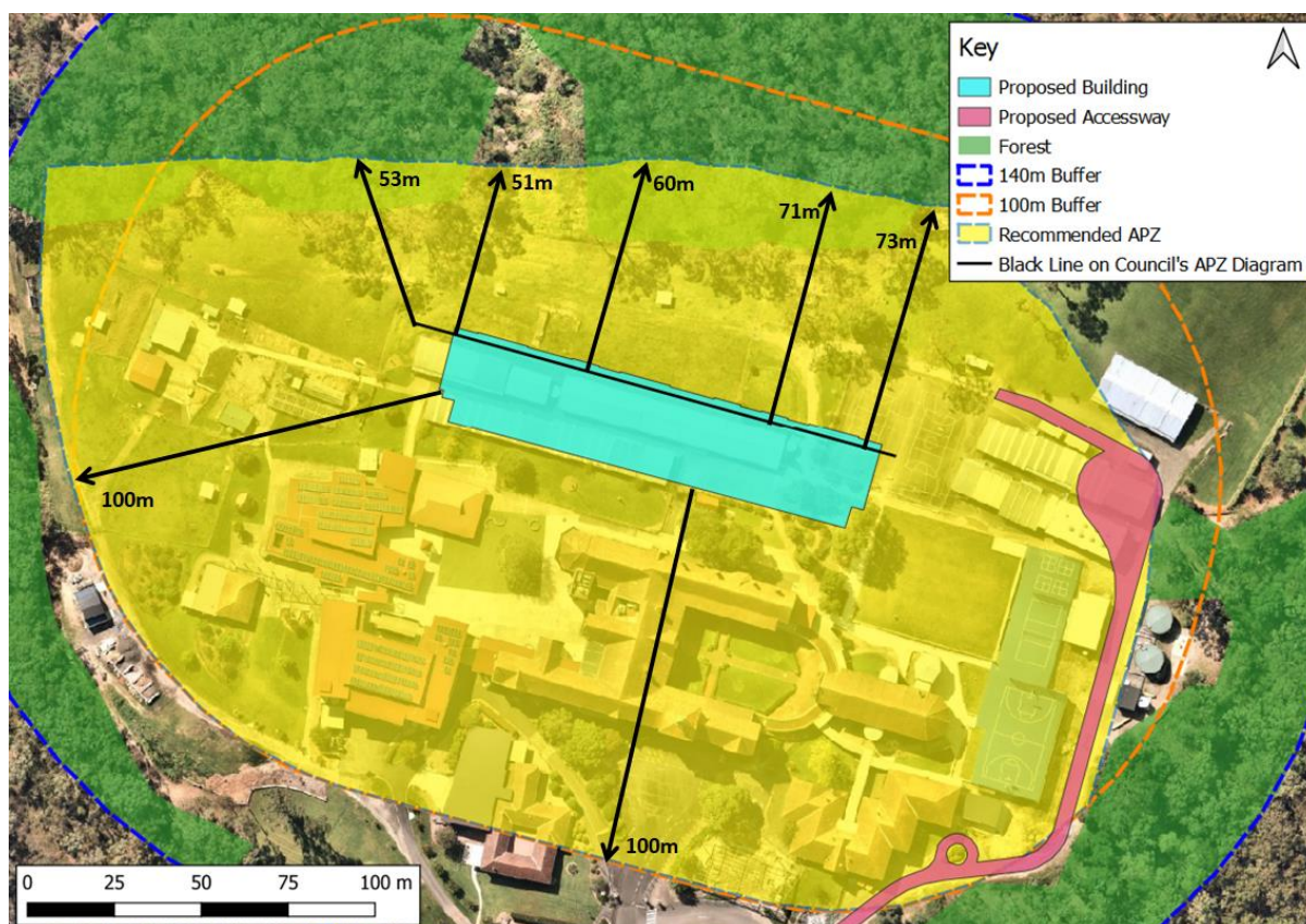
Figure 13. APZ Diagram. Source: NearMap (2022) and LiDAR (NSW Government 2022a) and Council letter dated 17/06/2022 with overlays by BFCS P/L
