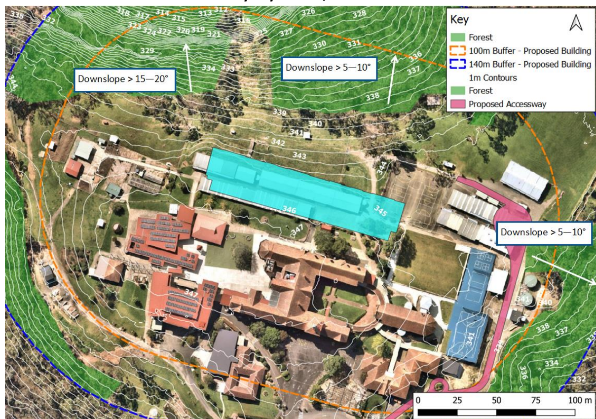
Figure 11. Slope Diagram. Source: NearMap (2022) and LiDAR (NSW Government 2022a) with overlays by BFCSP/L – 1m Contours
